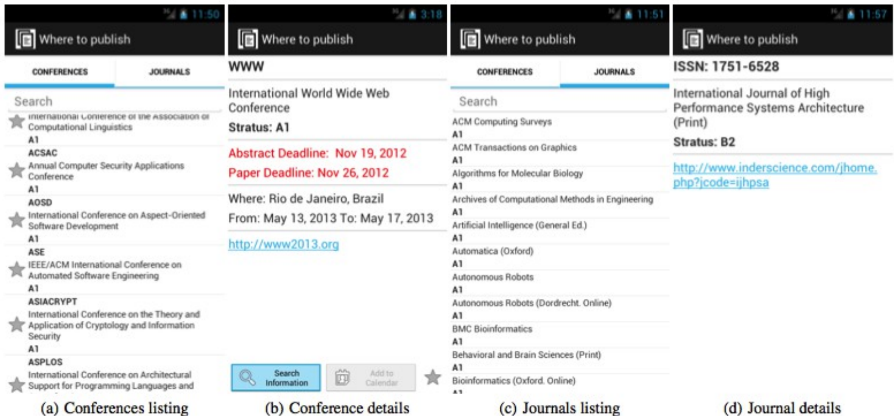
Figure 2: Where to publish mobile application screenshots
