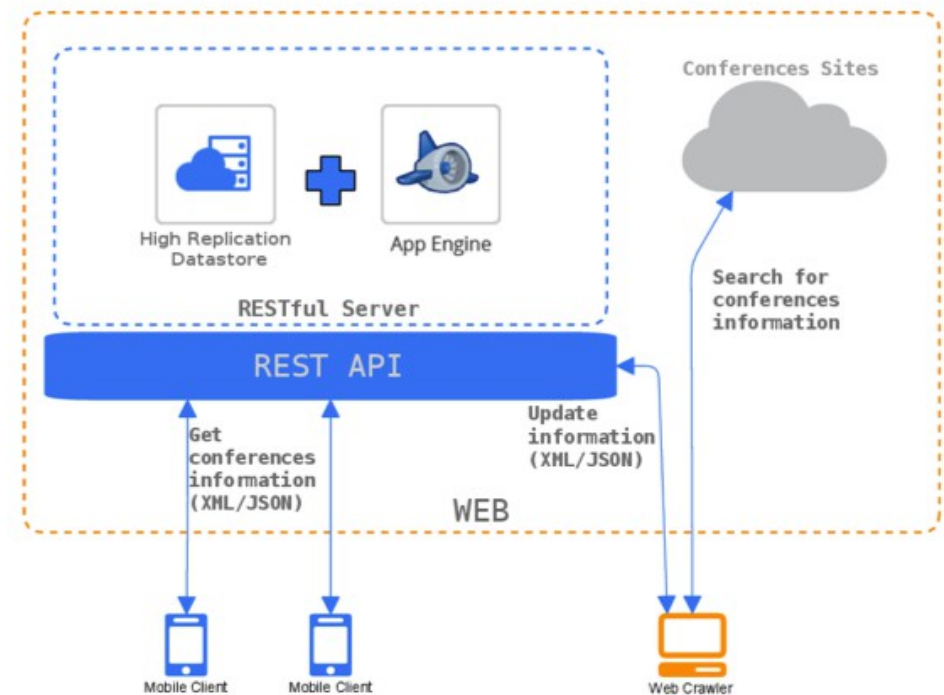
Figure 1: Where to Publish system diagram
